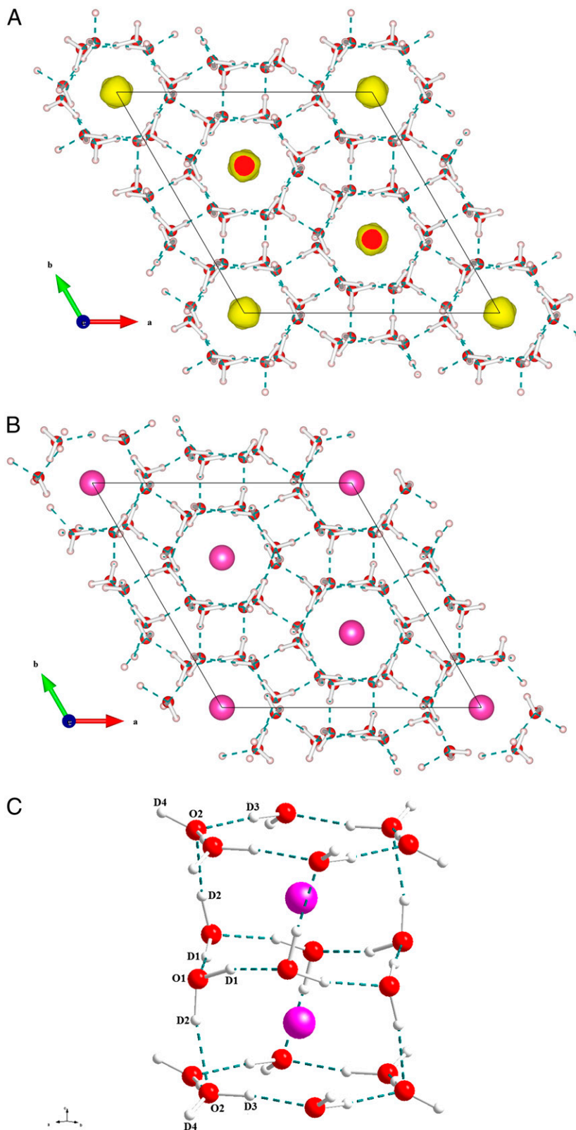
Fig. 3. (A) The difference Fourier nuclear density map without Ne atoms in ice cages shows that the incorporated Ne atoms occupy the center of D 2 O channels. The isosurface is at 7 fm 3 , as shown by the yellow surface. The red dots, which represents higher density of the isosurface, are the intersection of the yellow ball with the cutoff of the unit cell along the (001) plane. The red, white, and purple balls represent O, H, and Ne atoms, respectively (B and C). The D–O bonds within the D 2 O molecule are represented by solid white lines; the hydrogen bonds that connect different D 2 O molecules are represented by dashed green lines. (B) A top view of the refined crystal structure for Ne hydrate ( c direction). (C) A side view of the refined crystal structure for Ne hydrate. D1–O1–D2 are water molecules in the puckered ring. D1s connect the ring inside and D2s connect the adjacent flat ring. D3–O2–D4 are water molecules in the flat ring. D3s connect the ring inside and D4s connect different channels.
