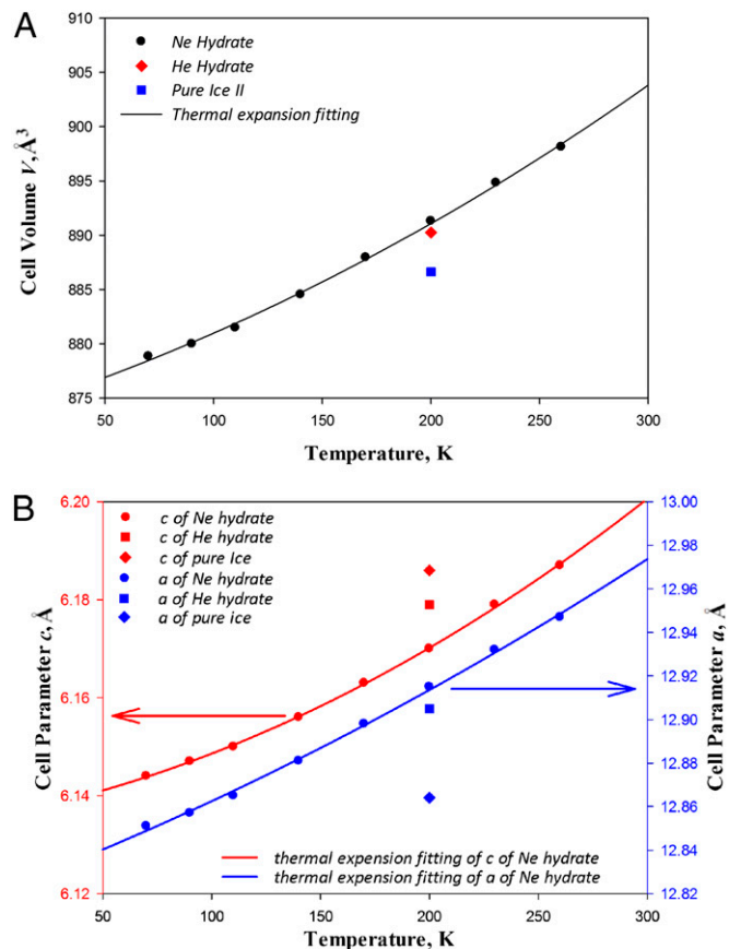
Fig. 2. Temperature dependence of cell parameters of Ne hydrate at 480 MPa (A, volume; B, lattice parameters a and c ). The data for pure ice II (11) and He hydrate (5) at 480 MPa and 200 K are also presented for comparison.
