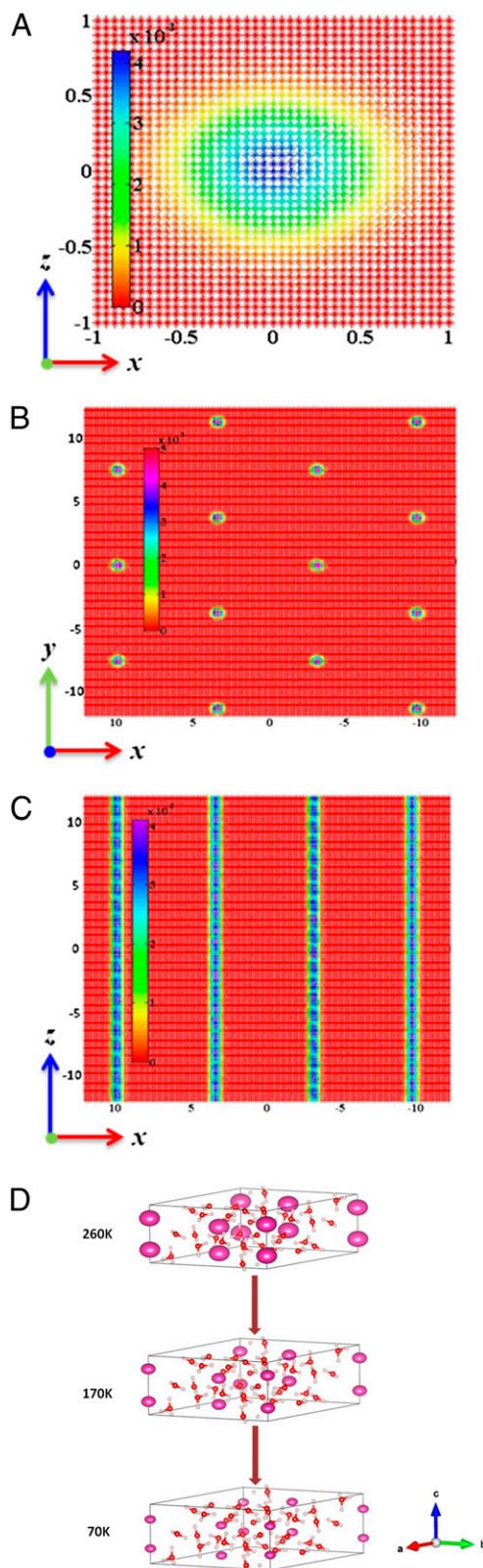
Fig. 5. (A) Projection of Ne local density distribution ( \times 10^3 ) in a single hydrate cage on the a – c ( x – z ) plane. (B) Projection of Ne global density distribution on the a – b ( x – y ) plane. (C) Projection of Ne global density distribution on the a – c ( x – z ) plane. The units in A, B, and C are angstroms. (D) The vibration of Ne atoms in D 2 O cages refined from neutron diffraction patterns at selected temperatures.
